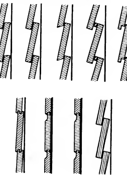
16 Horizontal cladding
